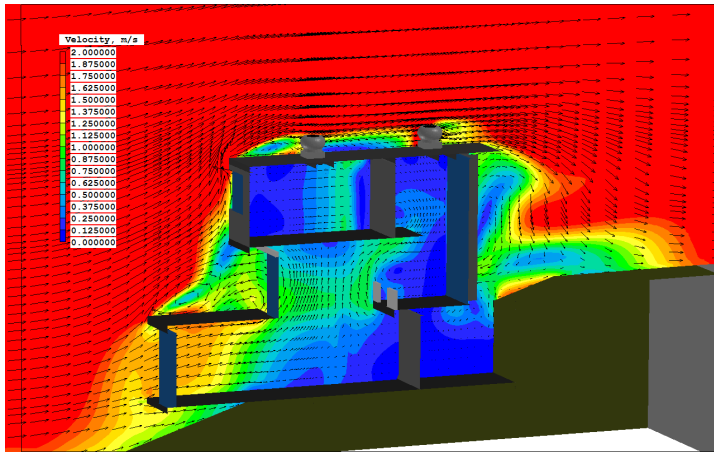
Figure 2. Velocity profile in x-plane
