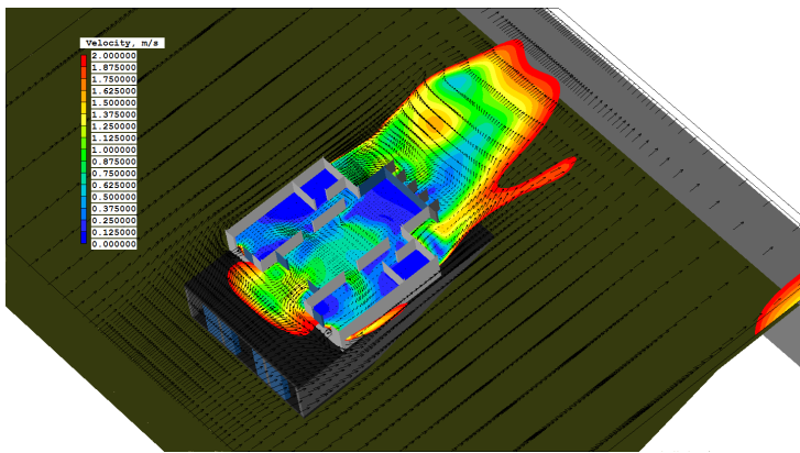
Figure 3. Velocity profile in z-plane
