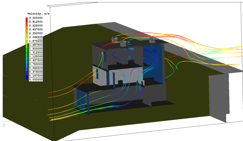
Figure 4. Streamline airflow in x-plane
