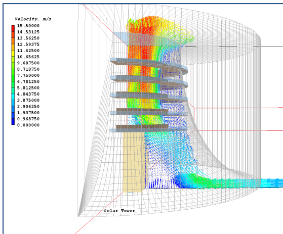
Velocity vectors
