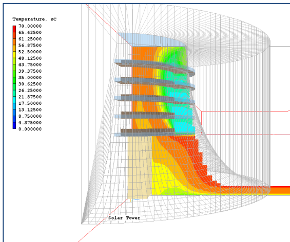
Temperature contours
