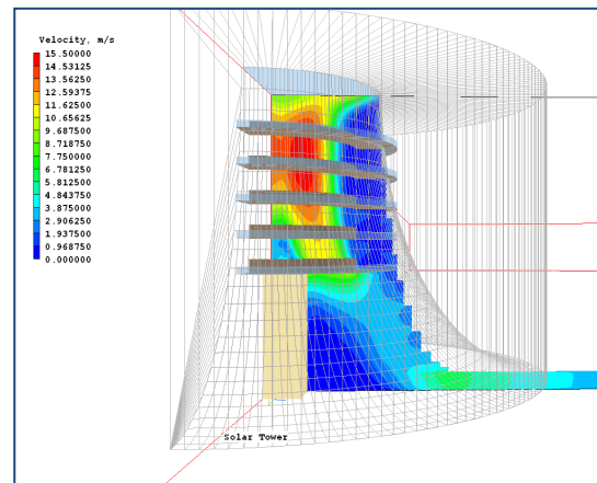
Velocity contours
